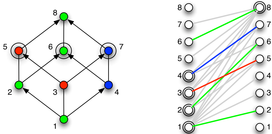
FIGURE 12. The equivalence of Dilworth’s and König’s theorems. The partially ordered set with 8 elements on the left is partitioned into 3 chains. This is the size of a minimum partition into chains, and is equal to the maximum size of an antichain (Dilworth’s theorem). The antichain is shown with double circles. On the right, the reachability graph constructed from the partially ordered set on the left is shown. The maximum matching corresponding to the chain partition consists of 5 edges and is equal in size to the number of vertices in a minimum vertex cover (König’s theorem). The vertex cover is shown with double circles. Note that 8=3+5 .
