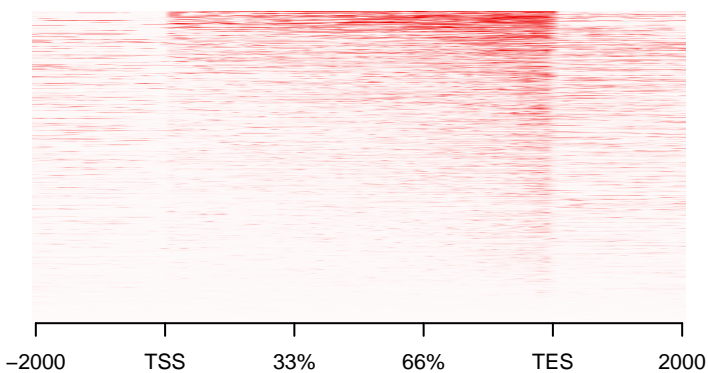
GMtr_1h_CHIPSeq_tr30m_recov1h_high
