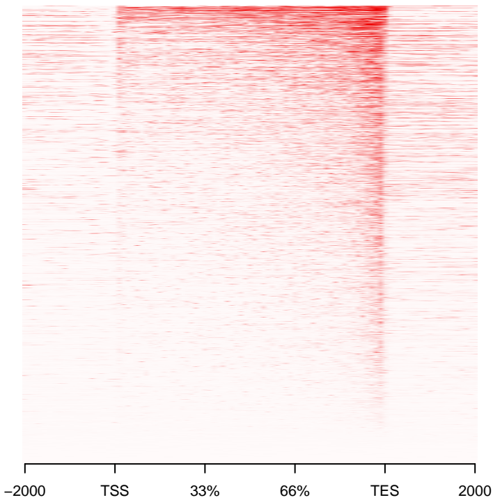
GMtr_1h_CHIPSeq_tr30m_recov1h_medium
