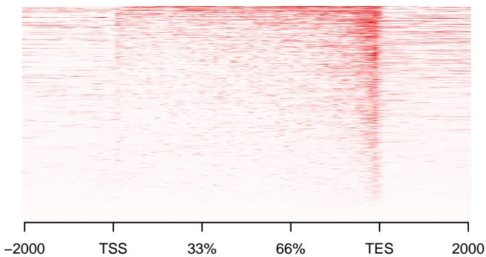
GMtr_1h_CHIPSeq_tr30m_recov1h_low
