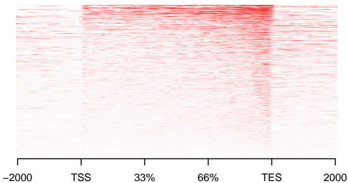
GMtr_0h_CHIPSeq_untr_high
