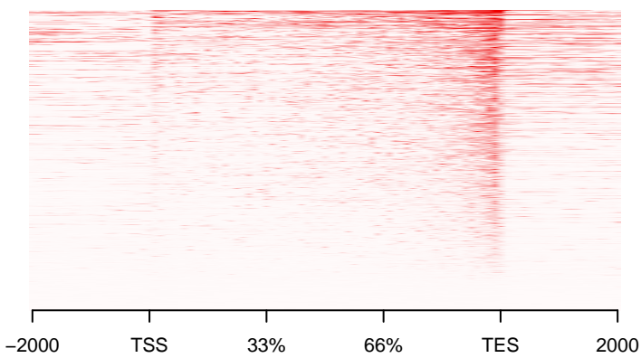
GMtr_0h_CHIPSeq_untr_low
