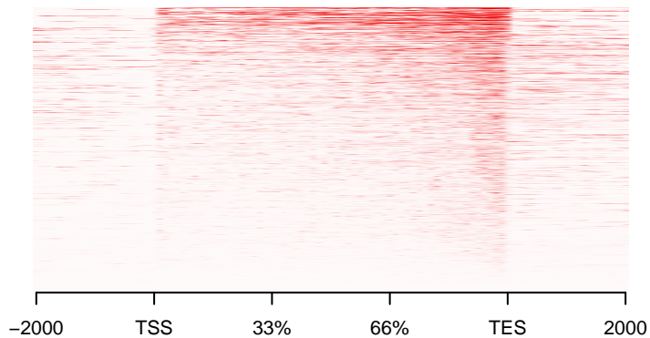
GMtr_0h_CHIPSeq_untr_high
