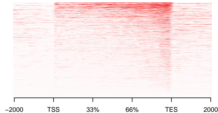
GM_untr_CHIPSeq_untr_high
