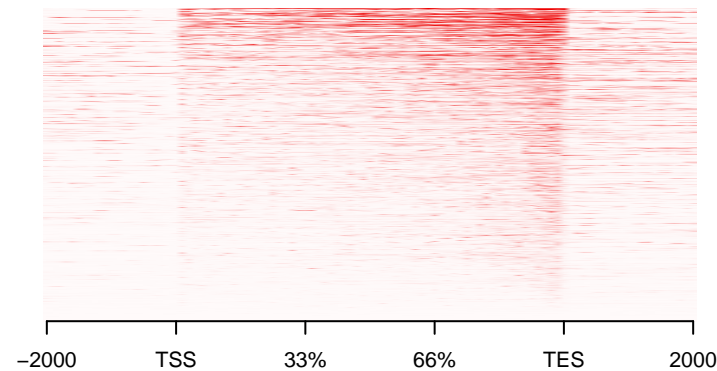
GMtr_3h_CHIPSeq_untr_high
