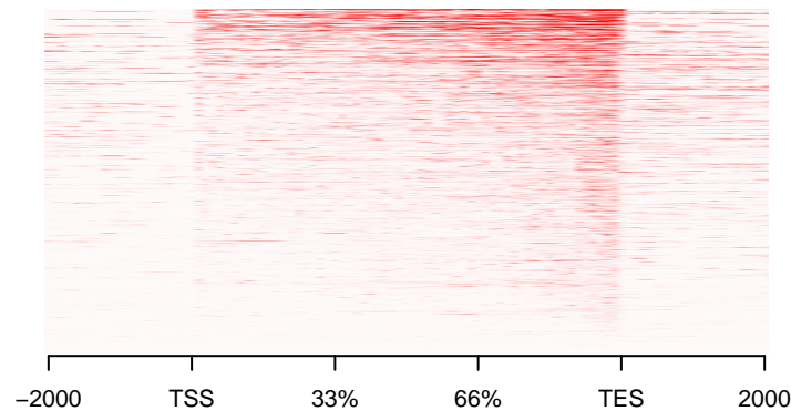
GMtr_1h_CHIPSeq_untr_high
