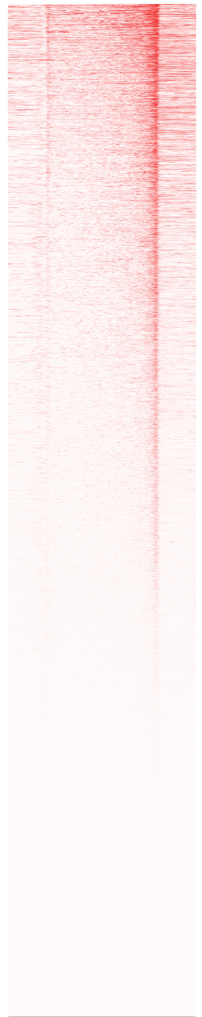
GM-tr-0h-longer-10k
