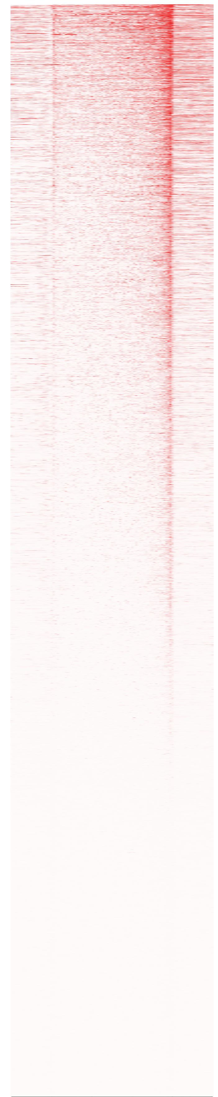
GM-tr-1h-longer-10k
