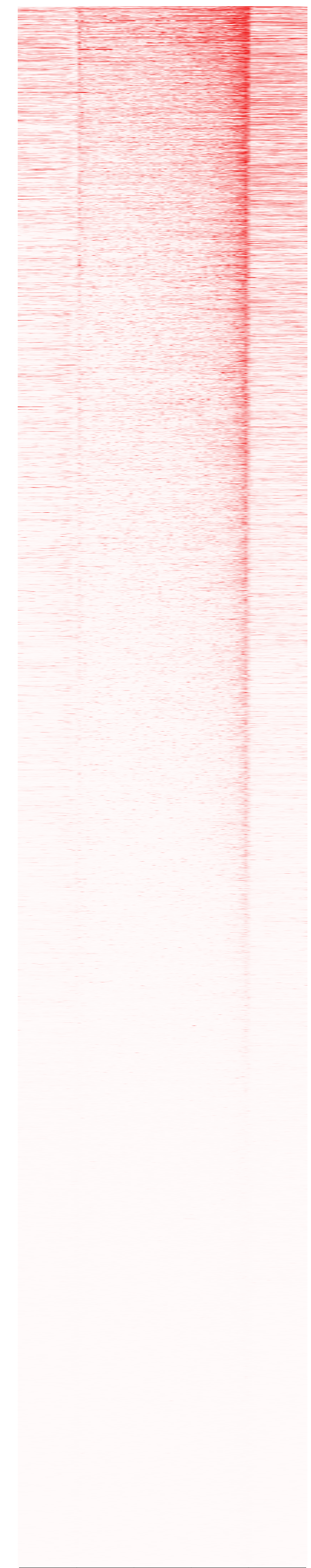
GM-tr-3h-longer-10k
