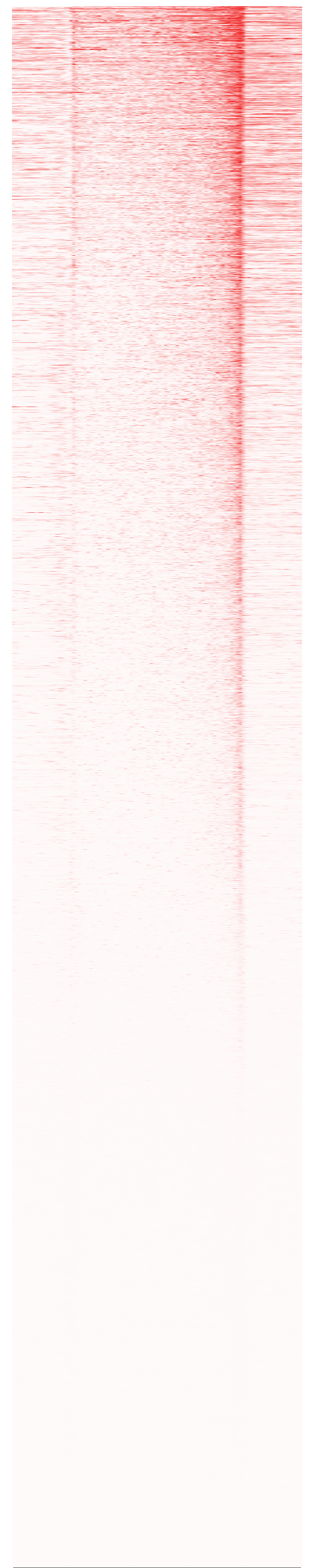
GM-untr-0h-longer-10k
