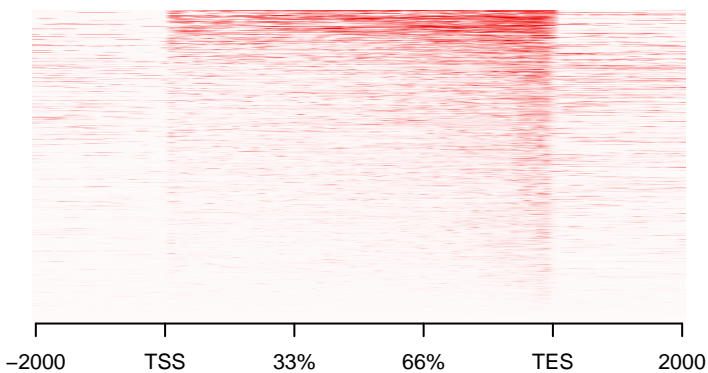
GM_untr_CHIPSeq_untr_high
