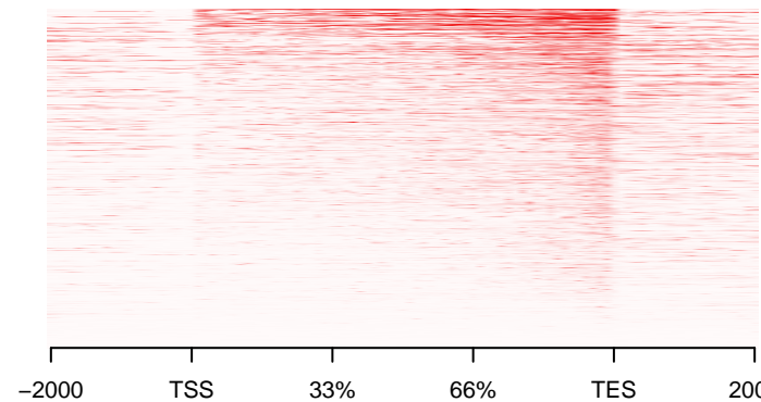
GMtr_3h_CHIPSeq_tr30m_recov1h_high
