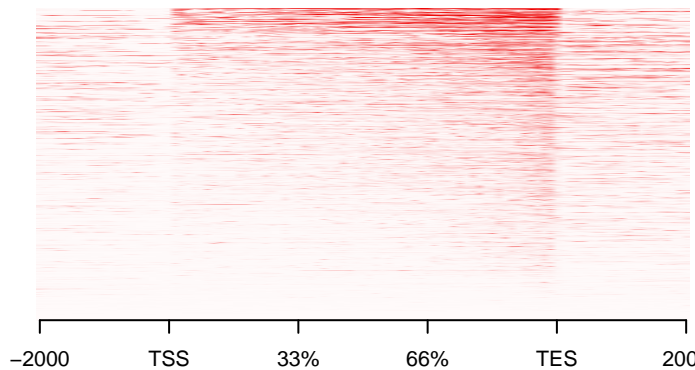
GMtr_1h_CHIPSeq_tr30m_recov1h_high
