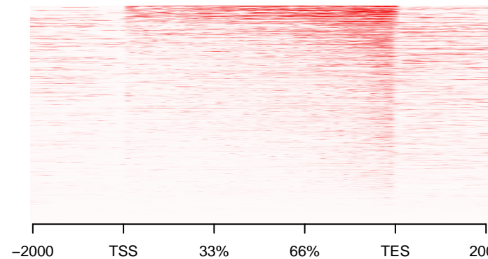
GM_untr_CHIPSeq_tr30m_recov1h_high
