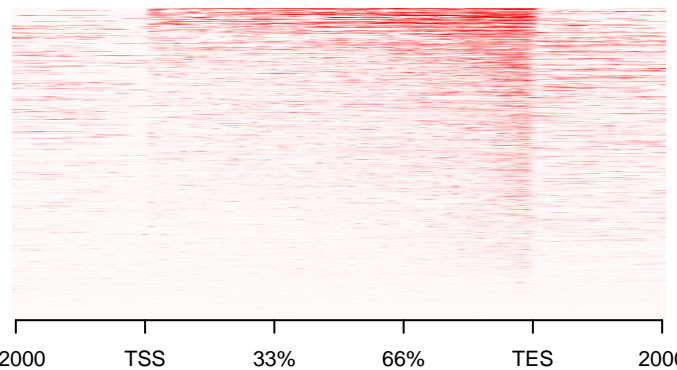
GMtr_0h_CHIPSeq_tr30m_recov1h_high
