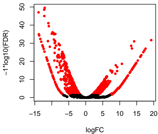
Volcano plot
