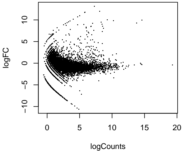
MA plot
