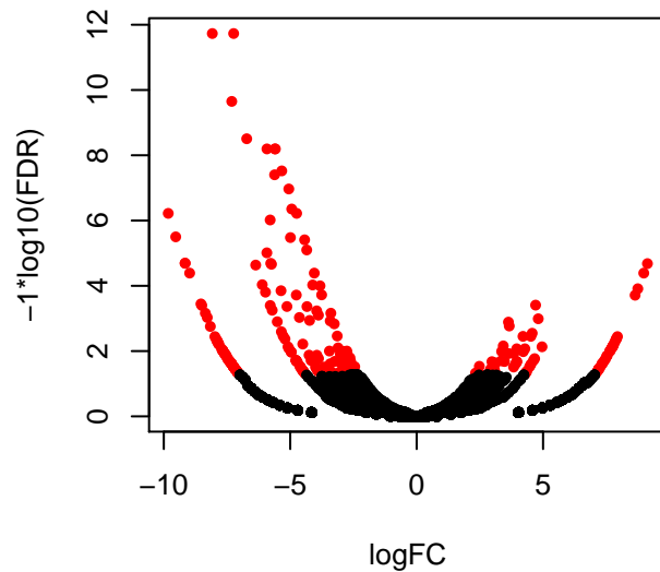
Volcano plot
